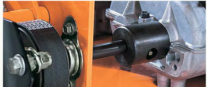
Five-speed Peerless transmission features nine-spline coupler shafts for durability and a wide selection of forward ground speeds.
